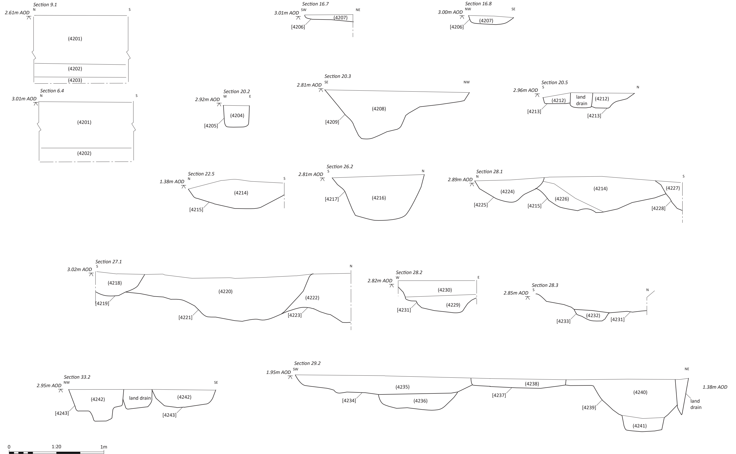
Figure 3.11: Detailed section drawings
