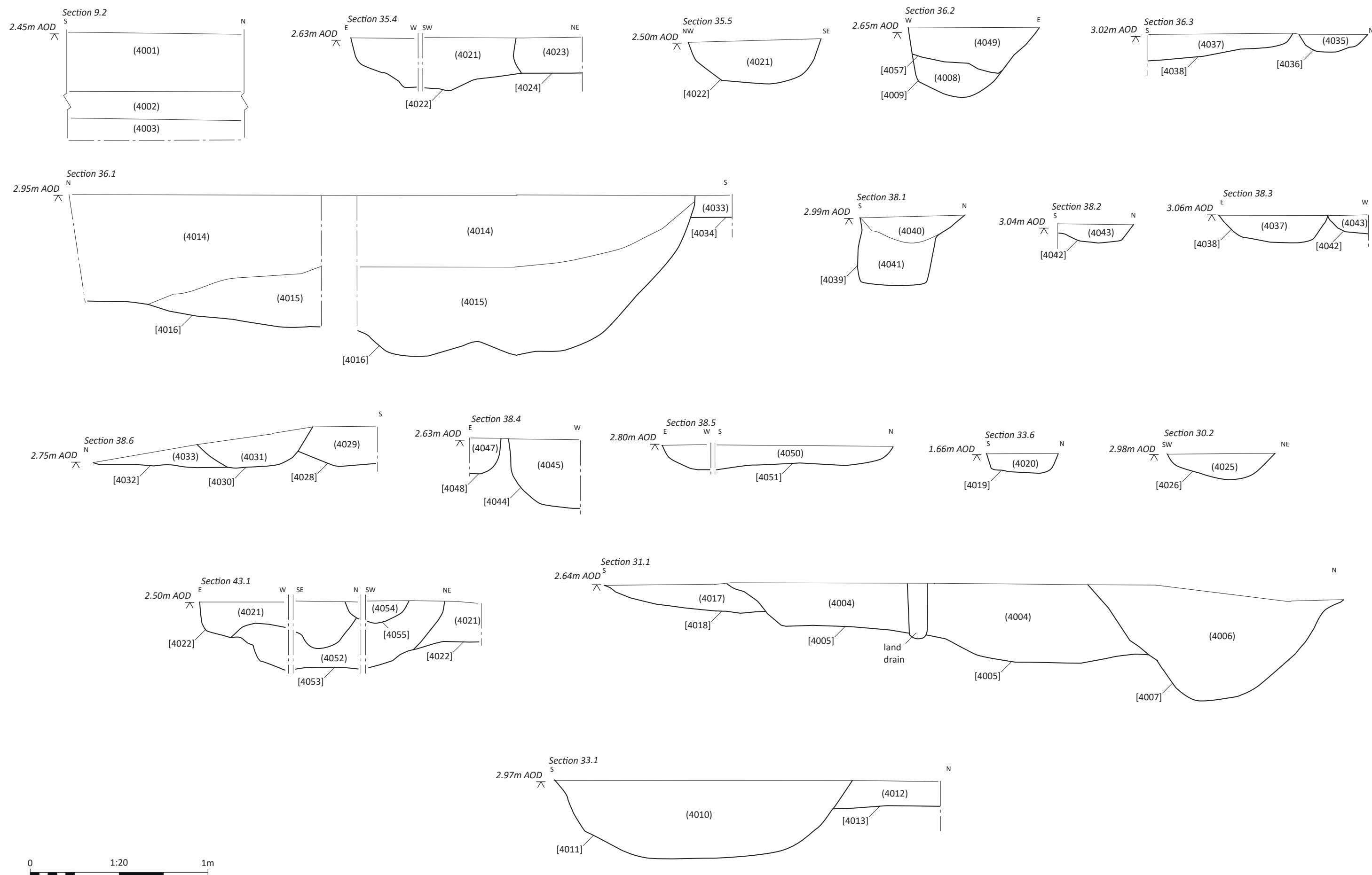
Figure 3.9: Detailed section drawings
