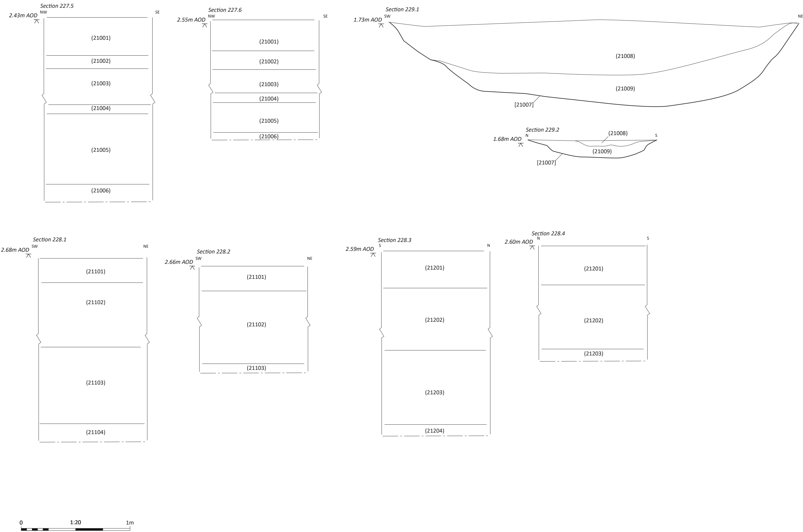
Figure 3.36: Detailed section drawings
