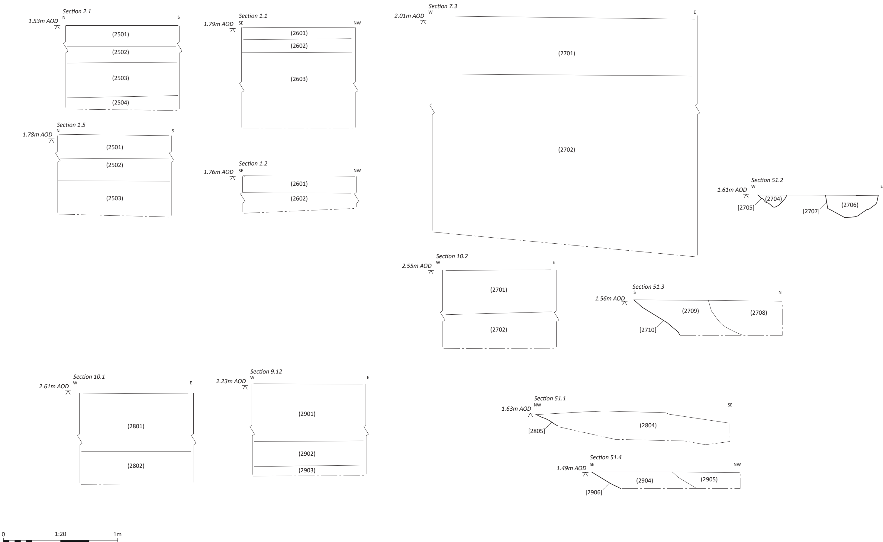
Figure 3.5: Detailed section drawings
