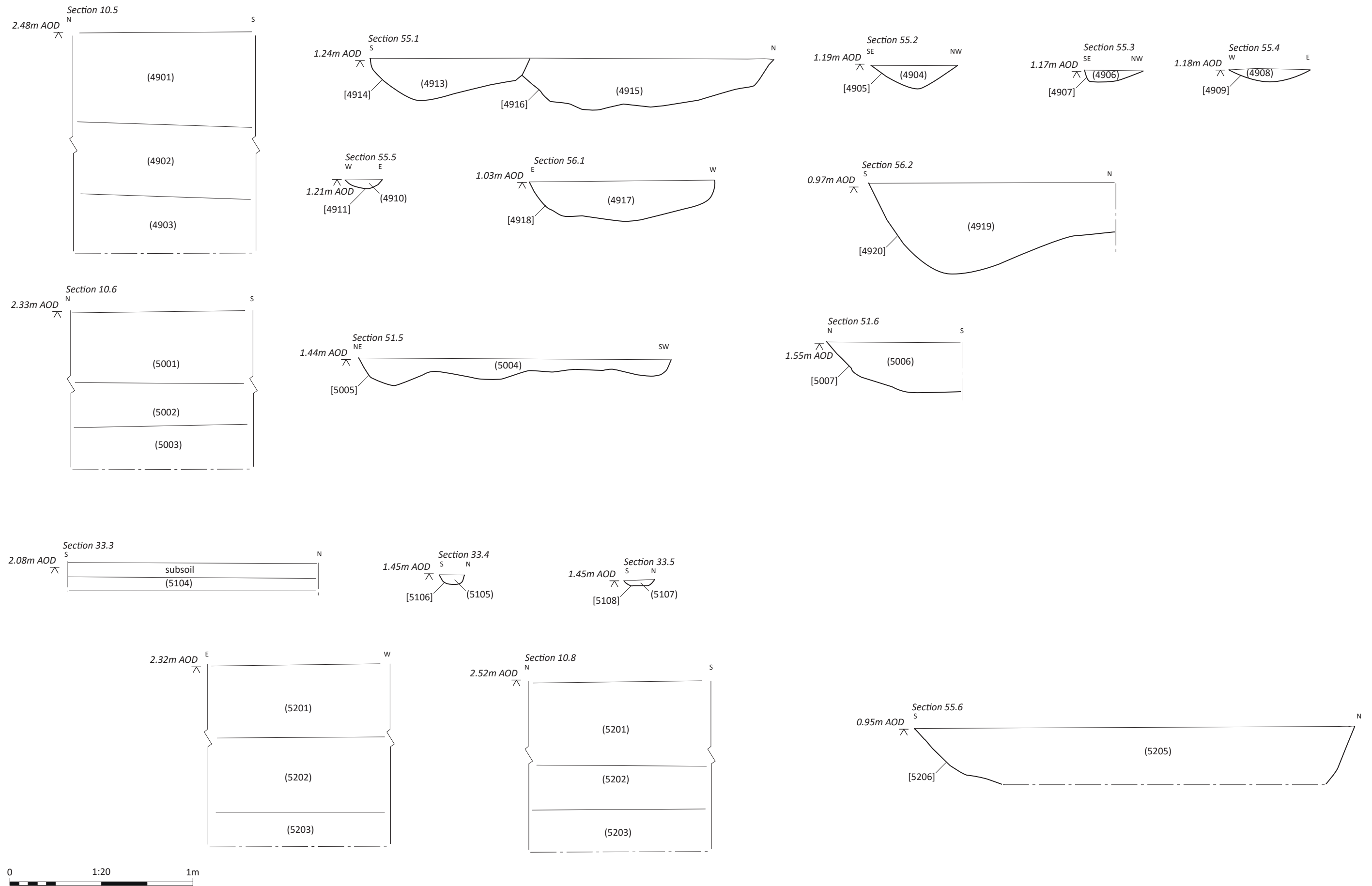
Figure 3.16: Detailed section drawings
