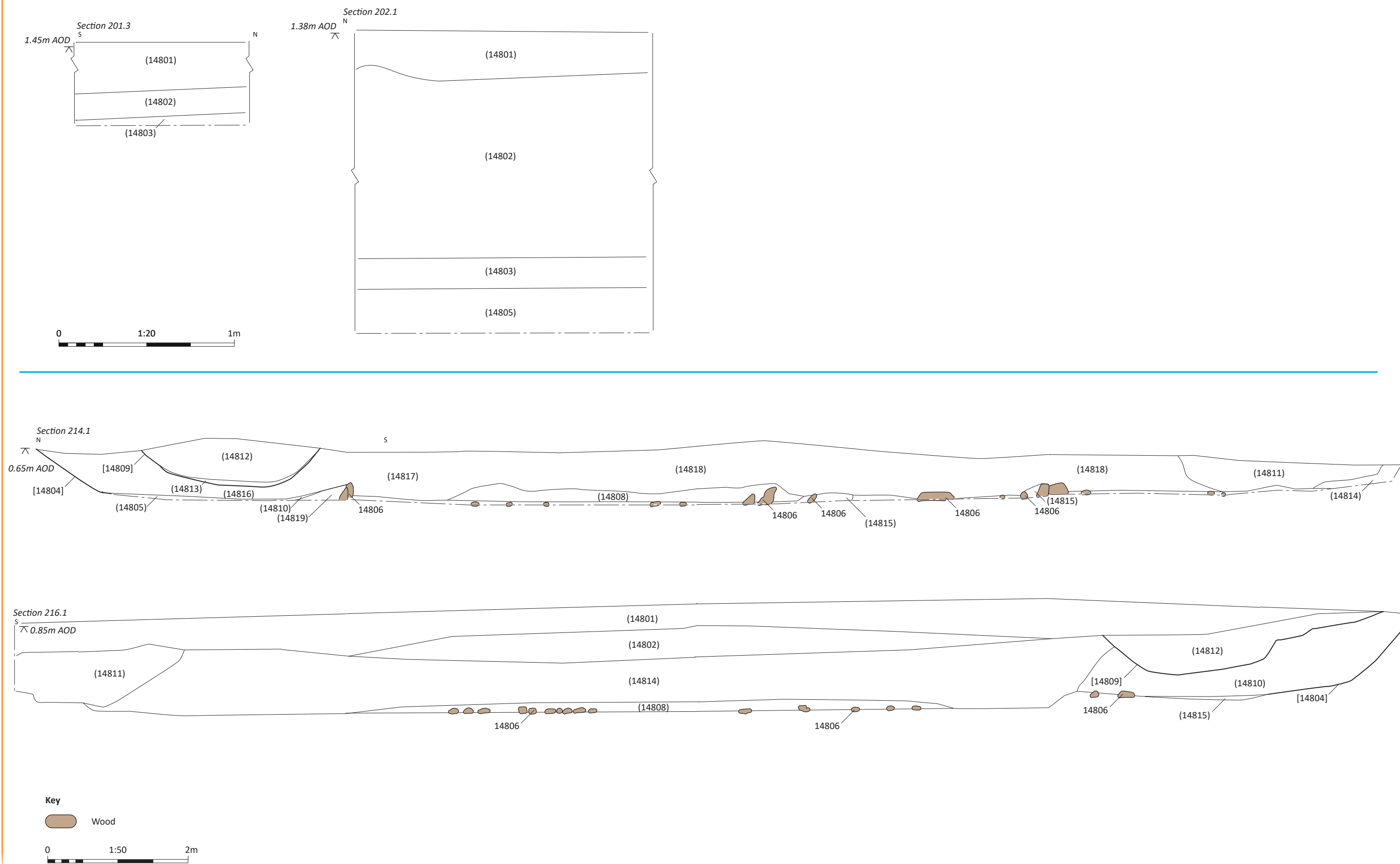
Figure 3.31: Detailed section drawings
