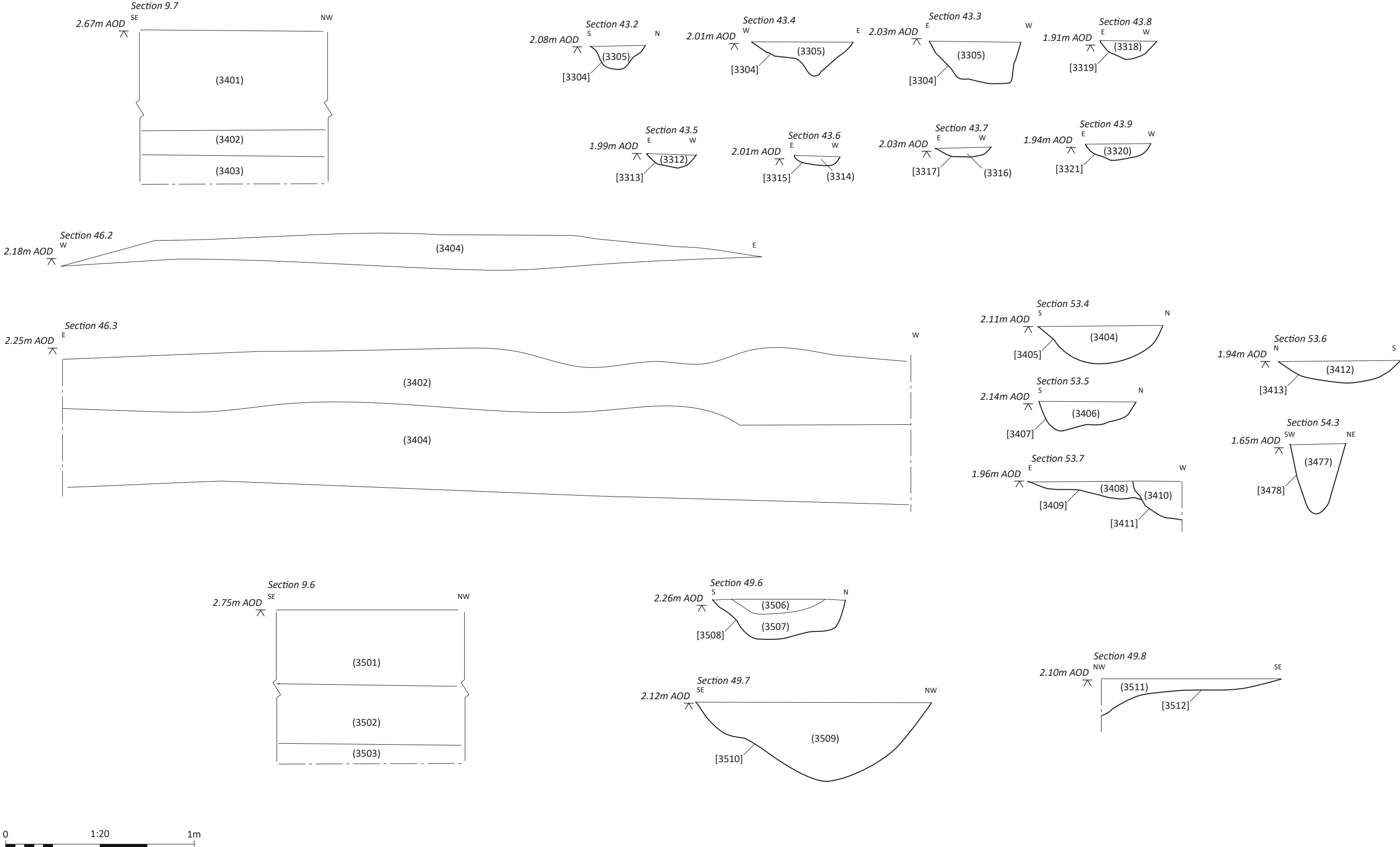
Figure 3.7: Detailed section drawings
