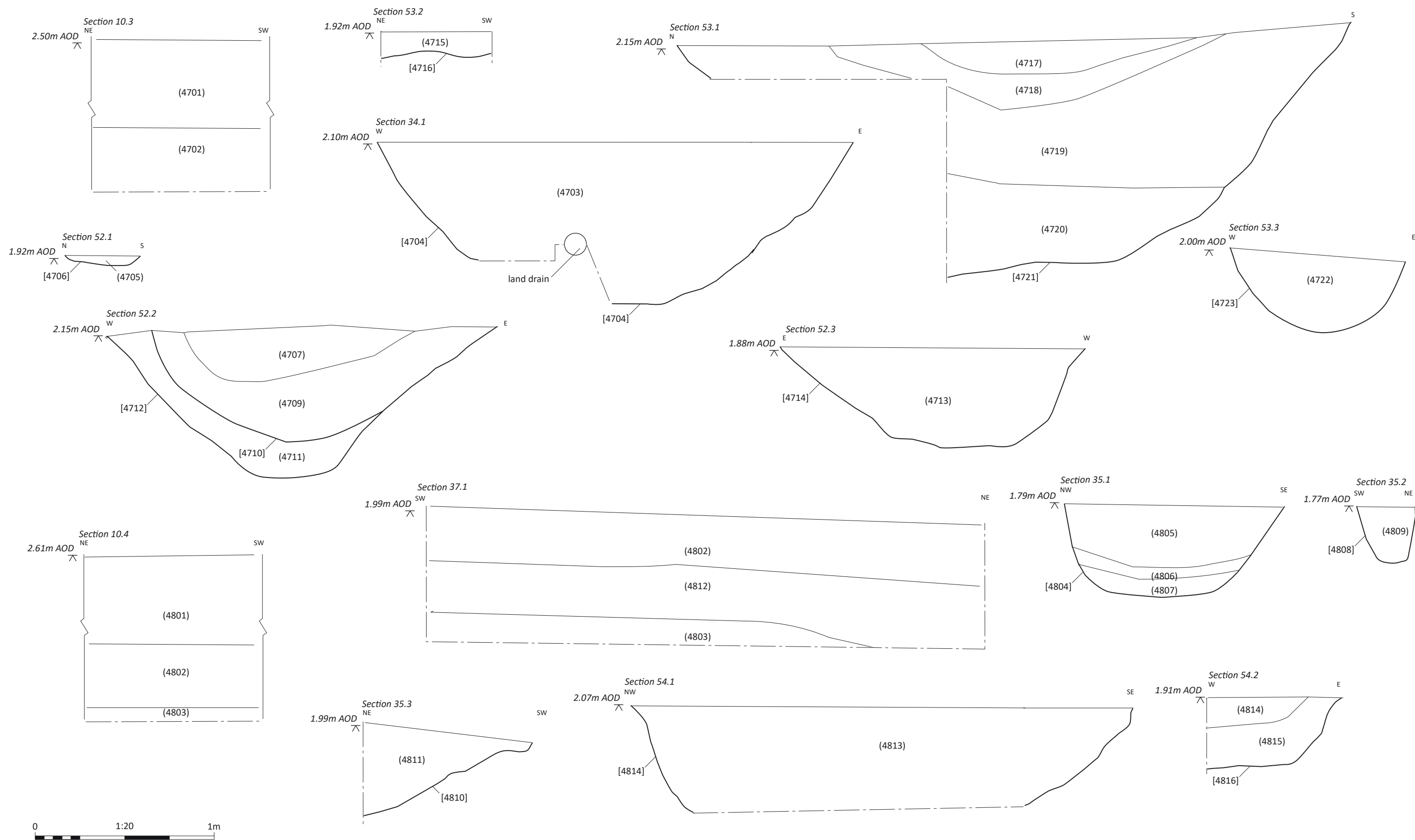
Figure 3.15: Detailed section drawings
