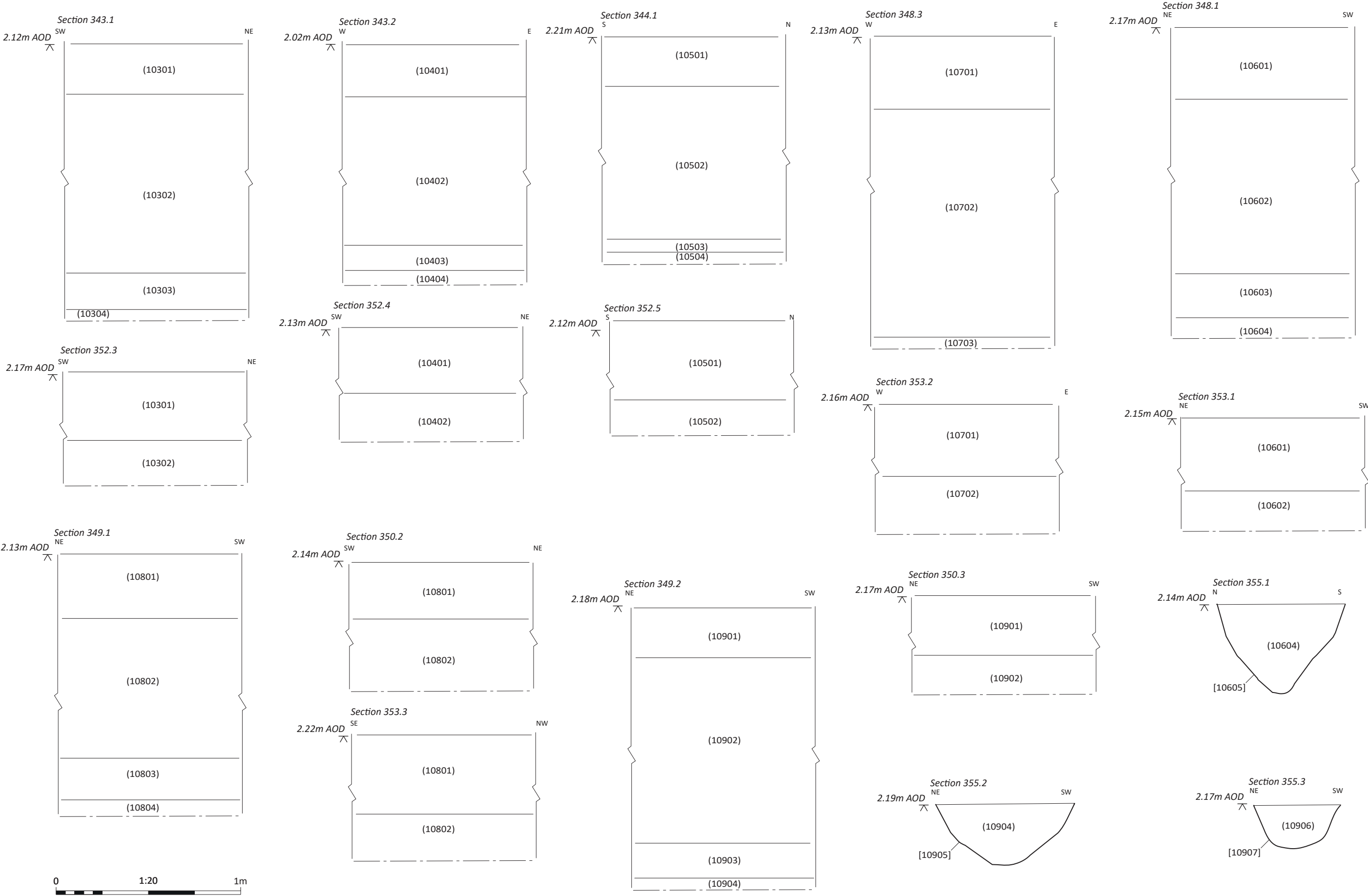
Figure 3.26: Detailed section drawings
