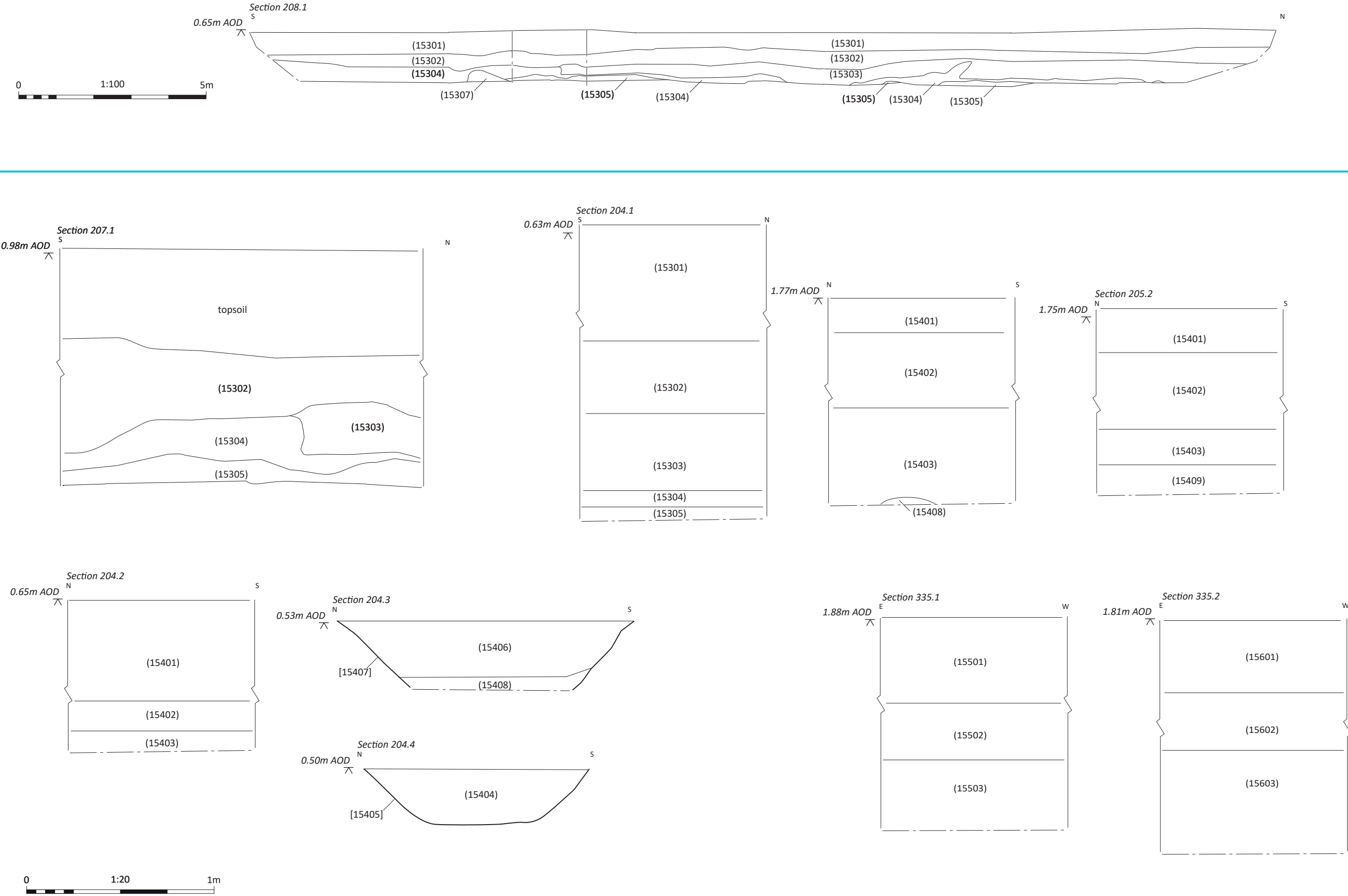
Figure 3.33: Detailed section drawings
